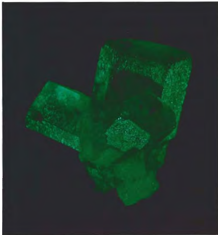
Figure 1. This 2.16-gram emerald crystal from the new Capoeirana locality shows the good crystallization that may be found there. The faceted stones, also from Capoeirana, weigh approximately 1.5–9 ct. Courtesy of Kalil Elawar; © Harold & Erica Van Pelt.
