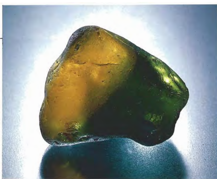
Figure 7. This 162.26-ct bicolored sapphire from Australia is unusual for both its large size and the sharp demarcation between the two zones. Photo by Shane McClure.
