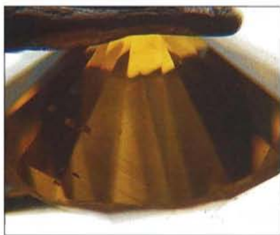
Figure 2. The brown graining in the synthetic diamond in figure 1 marks the cubic growth sectors. When examined from an oblique profile view with diffused transmitted light, this graining forms a pattern of concentric squares that could be confused with the phantom graining seen in some natural diamonds. Magnified 10 \times .
